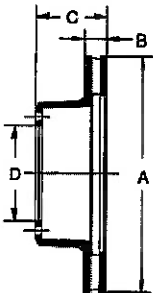
FLAT END Unitized Wheel End
